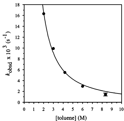
Figure 3. Plot of k_{\text{obsd}} vs [\text{toluene}] in 0.50 M TMCDA for the enolization of 1 by LiHMDS (0.10 M) in pentane cosolvent at -55\text{ }^{\circ}\text{C} . The curve depicts an unweighted least-squares fit to k_{\text{obsd}} = a[\text{toluene}]^b , where a = 4.6 \pm 0.4 \times 10^1 , b = -1.4 \pm 0.1 .
