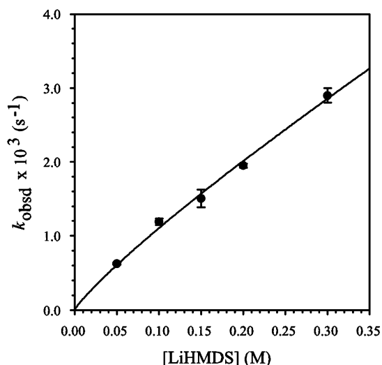
Figure 1. Plot of k obsd vs [LiHMDS] in 0.40 M trans -TMCDA/toluene solution for the enolization of 1 (0.005 M) by LiHMDS at –55 °C. The curve depicts the unweighted least-squares fit to k obsd = a [LiHMDS] b , where a = 8.0 ± 0.5 and b = 0.86 ± 0.4.
