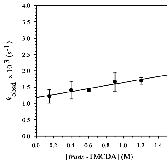
Figure 2. Plot of k_{\text{obsd}} vs [\text{trans-TMCDA}] in toluene cosolvent for the enolization of 1 (0.005 M) by LiHMDS (0.10 M) at -55\text{ }^{\circ}\text{C} . The curve depicts the results of an unweighted least-squares fit to k_{\text{obsd}} = a[\text{trans-TMCDA}] + b , where a = 4.6 \pm 0.1 \times 10^{-1} , b = 1.17 \pm 0.02 .
