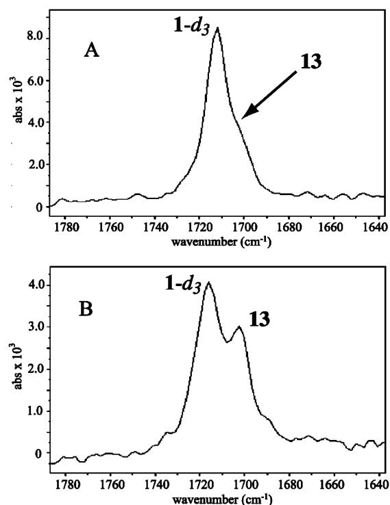
Figure 4. IR spectra showing free and LiHMDS-complexed 1-d 3 at -60\text{ }^{\circ}\text{C} with (a) LiHMDS (0.10 M), 1-d 3 (0.005 M), in 0.50 M TMEDA/toluene solution, and (b) LiHMDS (0.10 M), 1-d 3 (0.005 M), in 0.50 M TMEDA and 2.50 M toluene with pentane cosolvent.
