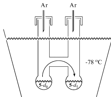
FIGURE 1. Vessel used for double-crossover experiment.
