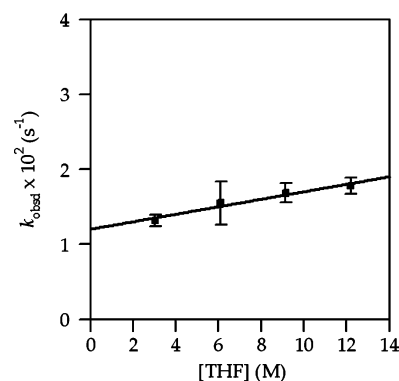
Figure 18. Plot of k_{\text{obsd}} vs [\text{THF}] in hexane cosolvent for the 1,4-addition of ester 1 (0.004 M) with LDA (0.10 M) in the presence of 1 mol % LiCl at -78^{\circ}\text{C} . The curve depicts an unweighted least-squares fit to y = k[\text{THF}] + k' [ k = (5.0 \pm 0.01) \times 10^{-4} ; k' = (1.2 \pm 0.1) \times 10^{-2} ].
