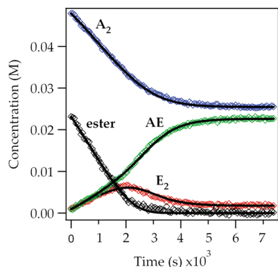
Figure 6. Time-dependent concentrations measured by ^6\text{Li} NMR spectroscopy using 0.05 M 3 (0.10 N) and 0.025 M 1 in 6.1 M THF at -78^\circ\text{C} . Legend: ester = 1 ; \text{A}_2 = LDA dimer 3 ; \text{E}_2 = enolate dimer 5a ; AE = enolate mixed dimer 4 . The curves represent a parametric fit to eqs 17–22 (described below). The best-fit values for the rate constants are listed in the Supporting Information.
