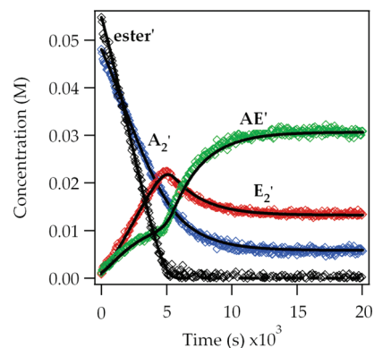
Figure 7. Time-dependent concentrations measured by ^6\text{Li} NMR spectroscopy using 0.05 M 3 (0.10 N) and 0.05 M ester 12 in 6.1 M THF at -78^\circ\text{C} . Legend: ester = 12 ; \text{A}_2 = LDA dimer 3 ; \text{E}_2 = enolate dimer of ester 12 ; \text{AE}' = enolate mixed dimer. The curves represent a parametric fit to eqs 17–22 (described below). The best-fit values for the rate constants are listed in the Supporting Information.
