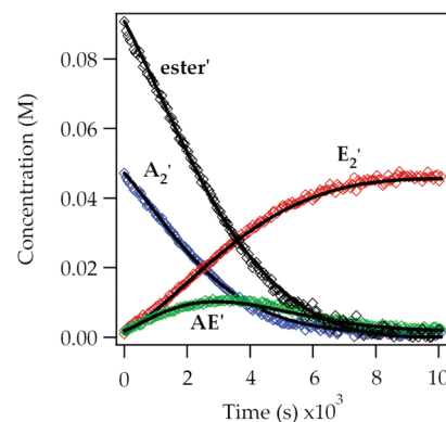
Figure 8. Time-dependent concentrations measured by ^6\text{Li} NMR spectroscopy using 0.05 M 3 (0.10 N) and 0.10 M 12 in 6.1 M THF at -78^\circ\text{C} . Legend: ester = 12 ; \text{A}_2 = LDA dimer 3 ; \text{E}_2' = enolate dimer of 12 ; \text{AE}' = enolate mixed dimer. The curves represent a parametric fit to eqs 17–22 (described below). The best-fit values for the rate constants are listed in the Supporting Information.
