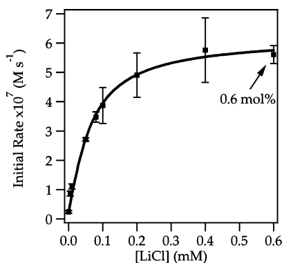
Figure 16. Plot of initial rate vs [\text{LiCl}] in THF (6.1 M) for the 1,4-addition of ester 1 (0.004 M) with LDA (0.10 M) at -78^{\circ}\text{C} . The 0.6 mol % notation is relative to the LDA concentration.
