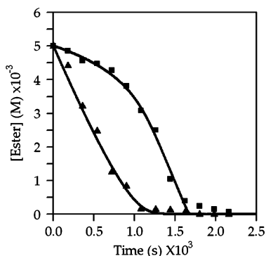
Figure 19. Plots of ester concentration vs time for the uncatalyzed 1,4-addition of LDA (0.10 M) to a mixture of esters 1 and 12 (0.005 M each) in THF (6.10 M) at -78\text{ }^{\circ}\text{C} : (■) ester 1 ; (▲) ester 12 . Results were analyzed by GC relative to a decane internal standard.
