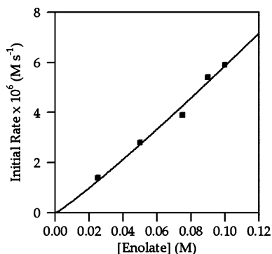
Figure 15. Plot of initial rate vs the concentration of enolate 5 for the condensation of LDA dimer 3 (0.10 M) with enolate dimer 5a in THF (6.10 M) at -78^{\circ}\text{C} . The curve depicts an unweighted least-squares fit to y = k[\text{enolate}]^n [ k = (7.4 \pm 0.3) \times 10^{-5} ; n = 1.10 \pm 0.14 ].
