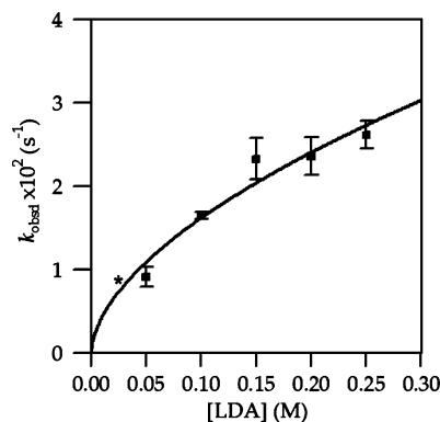
Figure 17. Plot of k_{\text{obsd}} vs [\text{LDA}] in THF (6.10 M) for the 1,4-addition of ester 1 (0.004 M) in the presence of 1 mol % LiCl at -78^{\circ}\text{C} . The curve depicts an unweighted least-squares fit to y = k[\text{LDA}]^n [ k = (6.01 \pm 0.04) \times 10^{-2} ; n = 0.57 \pm 0.08 ]. The asterisk denotes a point that departed markedly from pseudo-first-order conditions and was not included in the fit.
