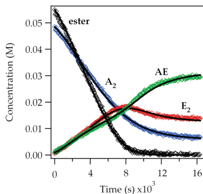
Figure 5. Time-dependent concentrations measured by ^6\text{Li} NMR spectroscopy using 0.05 M 3 (0.10 N) and 0.05 M 1 in 6.1 M THF at -78^\circ\text{C} . Legend: ester = 1 ; \text{A}_2 = LDA dimer 3 ; \text{E}_2 = enolate dimer 5a ; AE = enolate mixed dimer 4 . The curves represent a parametric fit to eqs 17–22 (described below). The best-fit values for the rate constants are listed in the Supporting Information.
