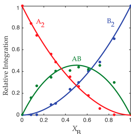
Figure 5. Job plot showing relative integration versus the measured 20 mole fraction of dimer for 0.10 M mixtures of [ 6 Li]3d (A) and [ 6 Li]3c (B) in 12.2 M THF at -80\text{ }^{\circ}\text{C} (see Figure 3).
