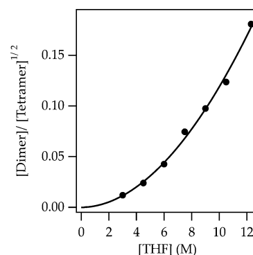
Figure 6. Plot of [\text{dimer}]/[\text{tetramer}]^{1/2} of 3d versus [\text{THF}] in toluene. The curve depicts an unweighted least-squares fit to y = K_{\text{eq}}[\text{THF}]^n [ K_{\text{eq}} = (1.4 \pm 0.3) \times 10^{-3} ; n = 1.94 \pm 0.09 ].
