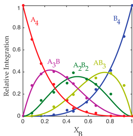
Figure 4. Job plot showing relative integration versus measured 20 mole fraction of tetramer for 0.10 M mixtures of [ 6 Li]3d (A) and [ 6 Li]3c (B) in 0.13 M THF at -80\text{ }^{\circ}\text{C} (see Figure 3).
