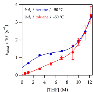
Figure 3. Plot of k_{\text{obsd}} vs THF concentration for the enolization of 0.0050 M oxazolidinone 9\text{-}d_2 with 0.10 M LiHMDS with THF at -50^\circ\text{C} in hexane (blue, curve A) and toluene (red, curve B). Curves depict an unweighted least-squares fit to the composite model described by eq 12 (vide infra). Curve A (hexane): [A]_0 is set at 0.10 M; K_{\text{eq}} = (4 \pm 3) \times 10^{-5} ; k_8 = (5 \pm 1) \times 10^{-3} ; k_9 = (5 \pm 5) \times 10^{-8} ; k_{10} = (1.9 \pm 0.6) \times 10^{-3} ; k_{11} = (4 \pm 1) \times 10^{-10} . Curve B (toluene): All parameters carried over from the fit from curve A; additionally, a = -4 \times 10^{-2} ; b = 9.2 \times 10^{-3} ; c = 1.04 ; and m = 1.2 .
