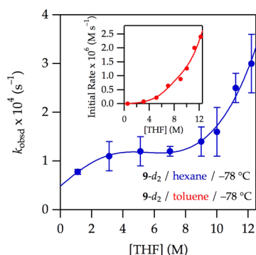
Figure 2. Plot of k_{\text{obsd}} vs THF concentration for the enolization of 0.0050 M oxazolidinone 9\text{-}d_2 with 0.10 M LiHMDS with THF in hexane or toluene cosolvent at -78^\circ\text{C} . Curves depict unweighted least-squares fits to the model described by eq 12 (vide infra). Curve A (hexane): [A]_0 is set at 0.10 M; K_{\text{eq}} = (1.1 \pm 1) \times 10^{-4} ; k_8 = (5 \pm 4) \times 10^{-4} ; k_9 = (8 \pm 20) \times 10^{-9} ; k_{10} = (2.2 \pm 1) \times 10^{-4} ; k_{11} = (7 \pm 3) \times 10^{-11} . Curve B (toluene) measured using initial rates: All parameters carried over from the fit from curve A; additionally, a = (-2 \pm 1) \times 10^{-4} ; b = (1.4 \pm 0.9) \times 10^{-4} ; c = 1.58 \pm 0.06 ; and m = 5 .
