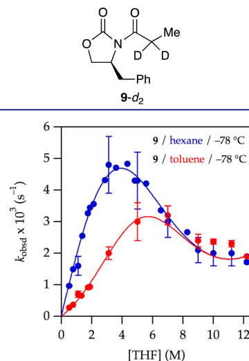
Figure 1. Plot of k_{\text{obsd}} vs tetrahydrofuran (THF) concentration 25 for the enolization of 0.0050 M oxazolidinone 9 with 0.10 M lithium hexamethyldisilazide (LiHMDS) with THF in hexane (curve A, blue) and toluene (curve B, red) at -78 °C. Curve depicts an unweighted least-squares fit to the composite model described by eq 12 (vide infra). Curve A (hexane): [A] 0 is set at 0.10 M; K_{\text{eq}} = (2.3 \pm 0.2) \times 10^{-4} ; k_8 = (3.9 \pm 0.1) \times 10^{-2} ; k_9 = (2 \pm 10) \times 10^{-8} ; k_{10} is set to 2.0 \times 10^{-4} ; k_{11} = (5 \pm 4) \times 10^{-10} . Curve B (toluene): All parameters carried over from the fit from curve A; additionally, a = -3.19 \times 10^{-5} ; b = 3.36 \times 10^{-5} ; c is set at 1.0; and m = 4.81 .
