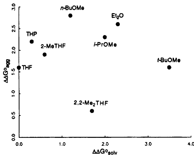
Figure 4. Plot of LiHMDS aggregation free energies ( \Delta\Delta G^\circ_{\text{agg}} , Table 3) vs LiHMDS dimer solvation energies ( \Delta\Delta G^\circ_{\text{solv}} , eqs 4 and 5, Table 3).
