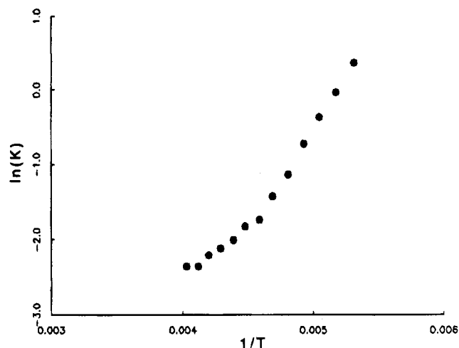
Figure 6. Temperature dependence of the monomer-dimer proportions (eq 1) for 0.1 M LiHMDS in pentane containing 75 equiv of THF per Li.
