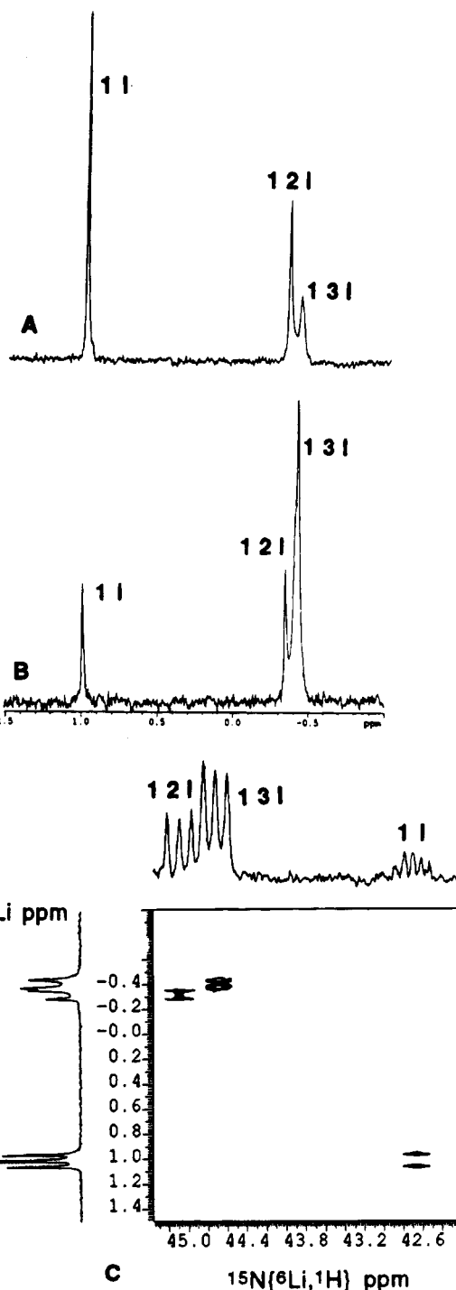
Figure 10. ^6Li NMR spectra of 0.1 M [^6Li]LiHMDS in pentane at -110 °C containing (A) 10 equiv of oxetane per Li and (B) 17 equiv of oxetane per Li. Spectrum (C) is a ^6Li - ^{15}N HMQC spectrum of 0.10 M [^6Li,^{15}N]LiHMDS in pentane containing with 13 equiv of oxetane per Li.
