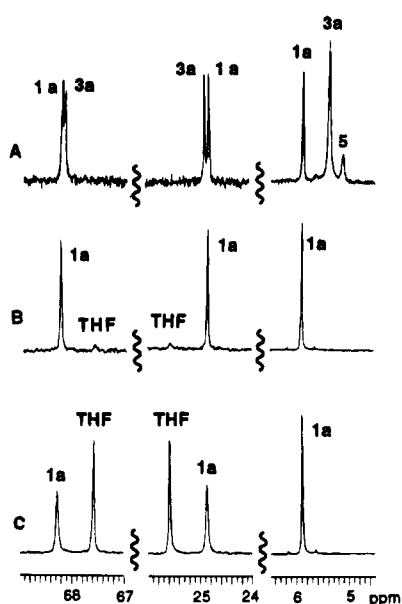
Figure 2. Partial 13 C NMR spectra of 0.10 M [ 6 Li]LiHMDS in toluene- d 8 at -100 °C with the following amounts of added ligand (per Li): (A) 0.7 equiv of THF; (B) 1.1 equiv of THF; (C) 2.0 equiv of THF.
