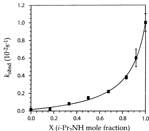
FIGURE 6. Plot of k_{\text{obsd}} vs i\text{-Pr}_2\text{NH} mole fraction in i\text{-Pr}_2\text{NH}/i\text{-Pr}_2\text{O}^{24} for the enolization of 1 (0.004 M) by LiHMDS (0.10 M) at -78^\circ\text{C} . The curve depicts an unweighted least-squares fit to y = (a + bx)/(1 + cx) , where a = (1 \pm 1) \times 10^{-5} , b = (1.2 \pm 0.2) \times 10^{-3} , c = -0.871 \pm 0.008 . K_A(i\text{-Pr}_2\text{NH}/i\text{-Pr}_2\text{O}) = 1 + c = 0.129 \pm 0.008 .
