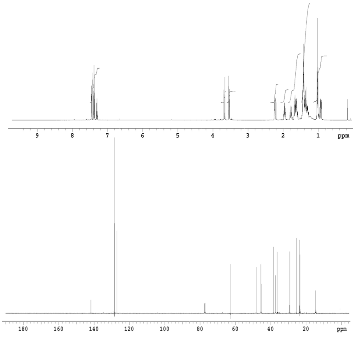
^1\text{H} and ^{13}\text{C} NMR Spectra (see p S14)
