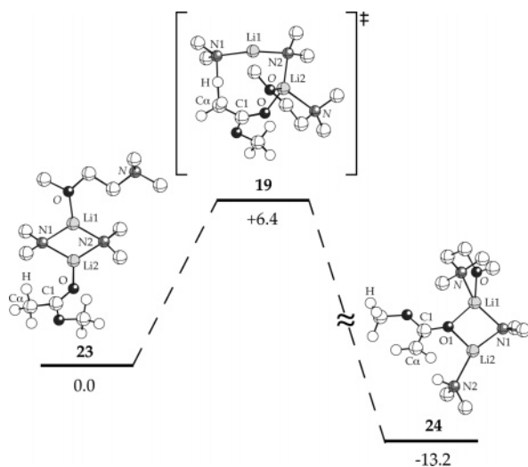
Chart 4. Calculated Reaction Coordinate for the Enolization of MeCO 2 Me by (Me 2 NLi) 2 /MeOCH 2 CH 2 NMe 2 .
