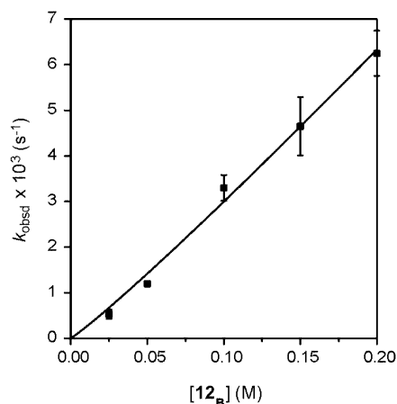
Figure 4. Plot of k_{\text{obsd}} vs [12_{\text{B}}] in \text{MeOCH}_2\text{CH}_2\text{NMe}_2 (0.5 M) and hexane cosolvent for the enolization of ester 2 (0.002 M) at -60 °C. The curve depicts the result of an unweighted least-squares fit to k_{\text{obsd}} = k[12_{\text{B}}]^n ( k = (3.6 \pm 0.5) \times 10^{-2} , n = 1.1 \pm 0.1 ).
