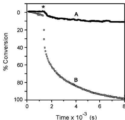
Figure 6. Plot of the percent conversion for the enolization of ester 2 (0.05 M) by LDA (0.1 M) at -78\text{ }^{\circ}\text{C} in hexane containing: (A, ■) n -BuOMe (1.0 M); (B, □) \text{MeOCH}_2\text{CH}_2\text{N}(i\text{-Pr})_2 (1.0 M). The asterisk indicates the addition of 0.2 equiv of ligand B relative to ester 2 .
