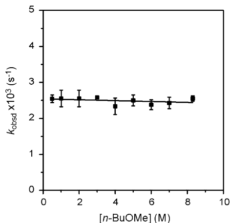
Figure 2. Plot of k_{\text{obsd}} vs [n\text{-BuOMe}] in hexane cosolvent for the enolization of 7 (0.004 M) by LDA (0.10 M) at 0 °C. The curve depicts an unweighted least-squares fit to k_{\text{obsd}} = k [n\text{-BuOMe}] + k' ( k = (-1 \pm 1) \times 10^{-5} , k' = (2.5 \pm 0.1) \times 10^{-3} ).
